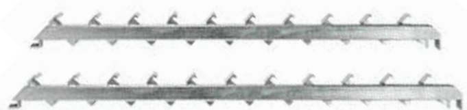
PSV-RL-9766R 10 Step Right Stair Stringer WT. 41.70 LBS
