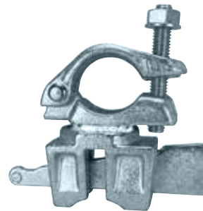
PSV-RL-9913 Ridge Adapter Wedge Coupler WT. 3.12 LBS
