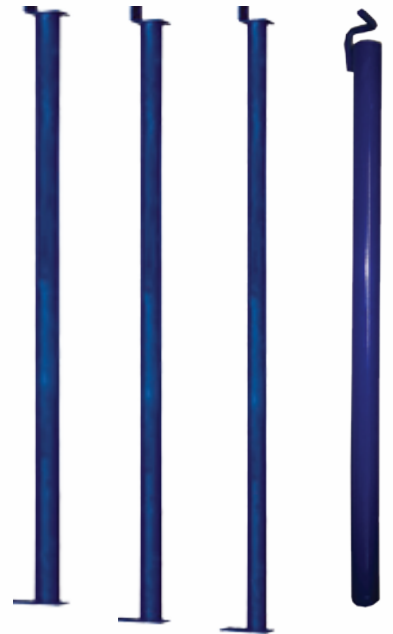
PSV-952 3' Tube Wall Tie WT. 5.20 LBS PSV-953 4' Tube Wall Tie WT. 6.80 LBS PSV-951 5' Tube Wall Tie WT. 7.80 LBS PSV-956 3' Tube Wall Tie W/Hooks WT. 6.20 LBS
