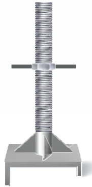
PSV-5161 25k Screw Jack with 6 X 6 X .500 J-Head WT. 14.64 LBS
