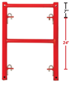
PSV-708 2' X 3' Shoring Frame WT. 28.00 LBS
