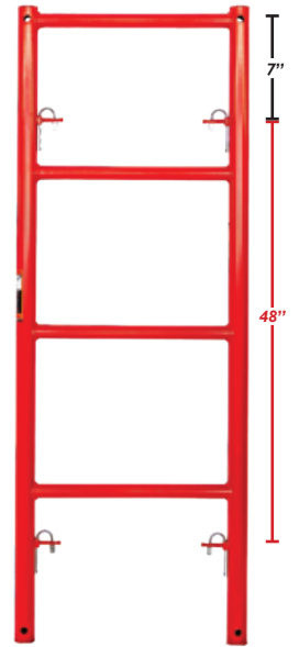
PSV-706 2' X 6' Shoring Frame WT. 53.40 LBS
