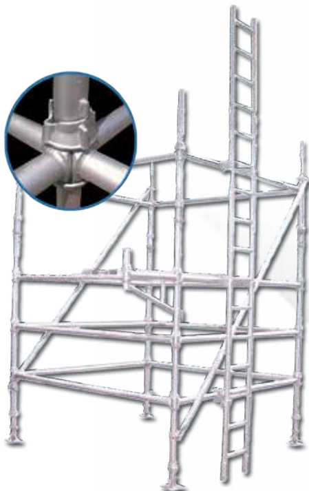
CUP Lock
