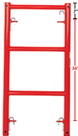
PSV-702 2' X 4' Shoring Frame WT. 38.20 LBS
