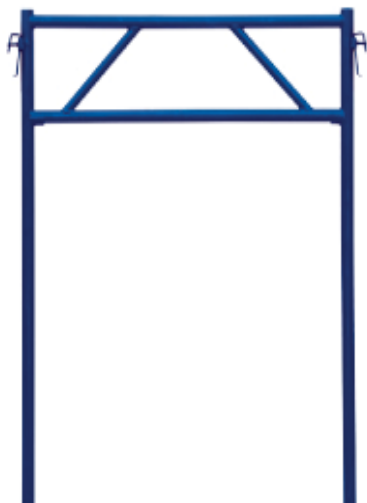
PSV-890 4' X 5'4" SX Extension Frame WT. 52.03 LBS
