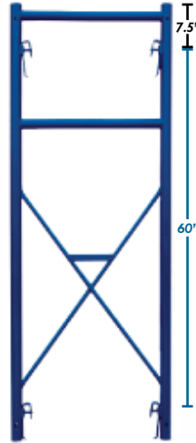
PSV-881 2' X 6' SX Base Frame WT. 54.38 LBS
