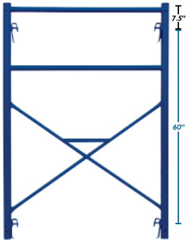
PSV-880 4' X 6' SX Base Frame WT. 65.25 LBS
