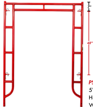
PSV-636AC 3' X 6'7" W-Style Walk-Thru Frame (3 Rung) WT. 42.35 LBS
