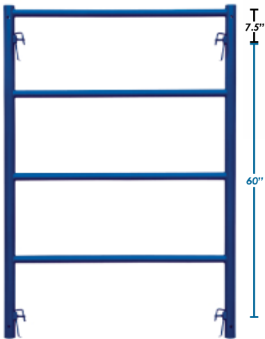
PSV-885 4' X 6' SX Base Frame (Ladder Style) WT. 66.35 LBS
