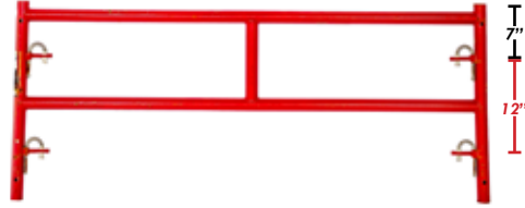
PSV-408A 5' X 2'1" W-Style Single Ladder WT. 25.01 LBS
