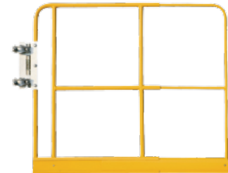
PSV-802 42" Expandable Access Gate W/ Toeboard WT. 32.20 LBS
