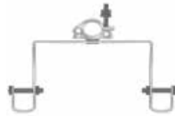
PSV-CL-8907 Cup Lock Ladder Bracket (14" Wide) WT. 6.09 LBS
