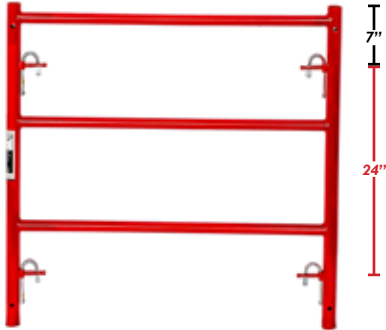
PSV-407A 3' X 3'1" W-Style Single Ladder WT. 21.80 LBS
