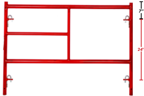
PSV-409A 5' X 3'1" W-Style Single Ladder WT. 30.40 LBS
