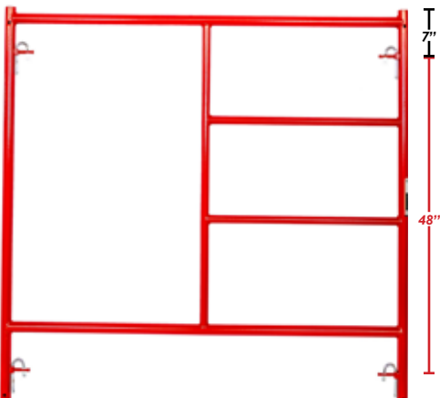
PSV-419A 5' X 5'1" W-Style Double Ladder WT. 41.20 LBS
