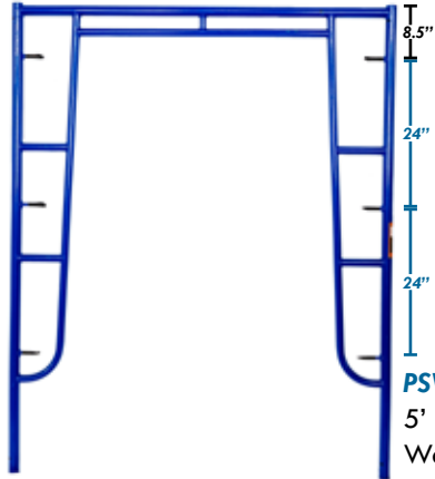
PSV-601B 3' X 6'4" S-Style Walk-Thru Frame WT. 41.40 LBS
