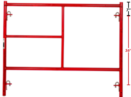
PSV-410A 5' X 4'1" W-Style Single Ladder WT. 35 LBS
