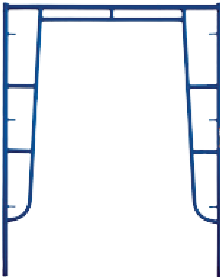
PSV-610B 5'X6'4" WALK THRU FRAME WT. 46.60 LBS
